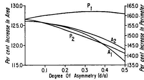
FIGURE 10 Per cent increase in surface area and perimeter (see text) as a function of asymmetry.
